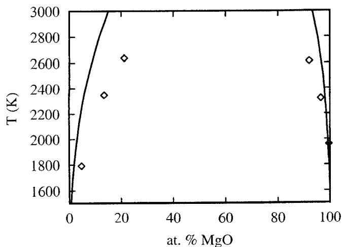
Fig. 5 Calculated (lines) and experimental (diamonds) phase diagrams of the CaO-MgO system
