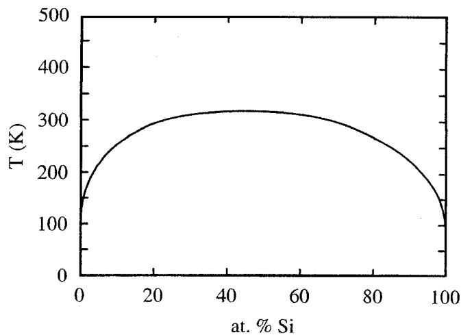
Fig. 3 Calculated phase diagram of Si-Ge system
