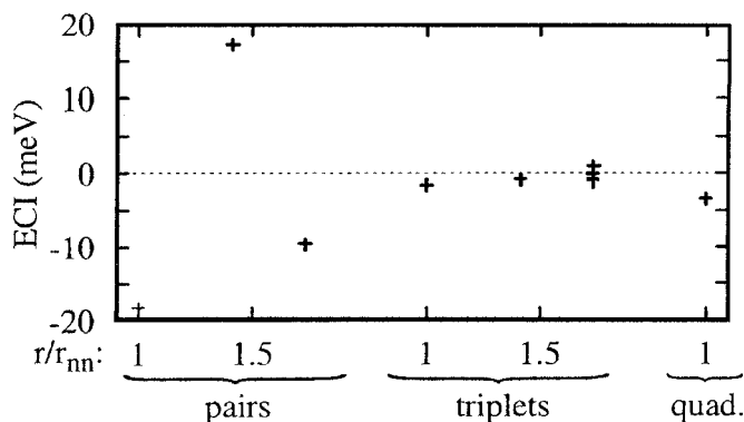
Fig. 4 Calculated ECI as a function of cluster diameter for the CaO-MgO system
